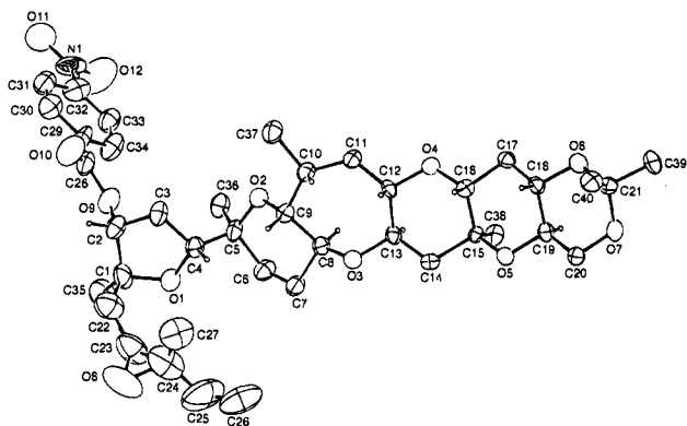
Figure 2. ORTEP drawing of 91.
